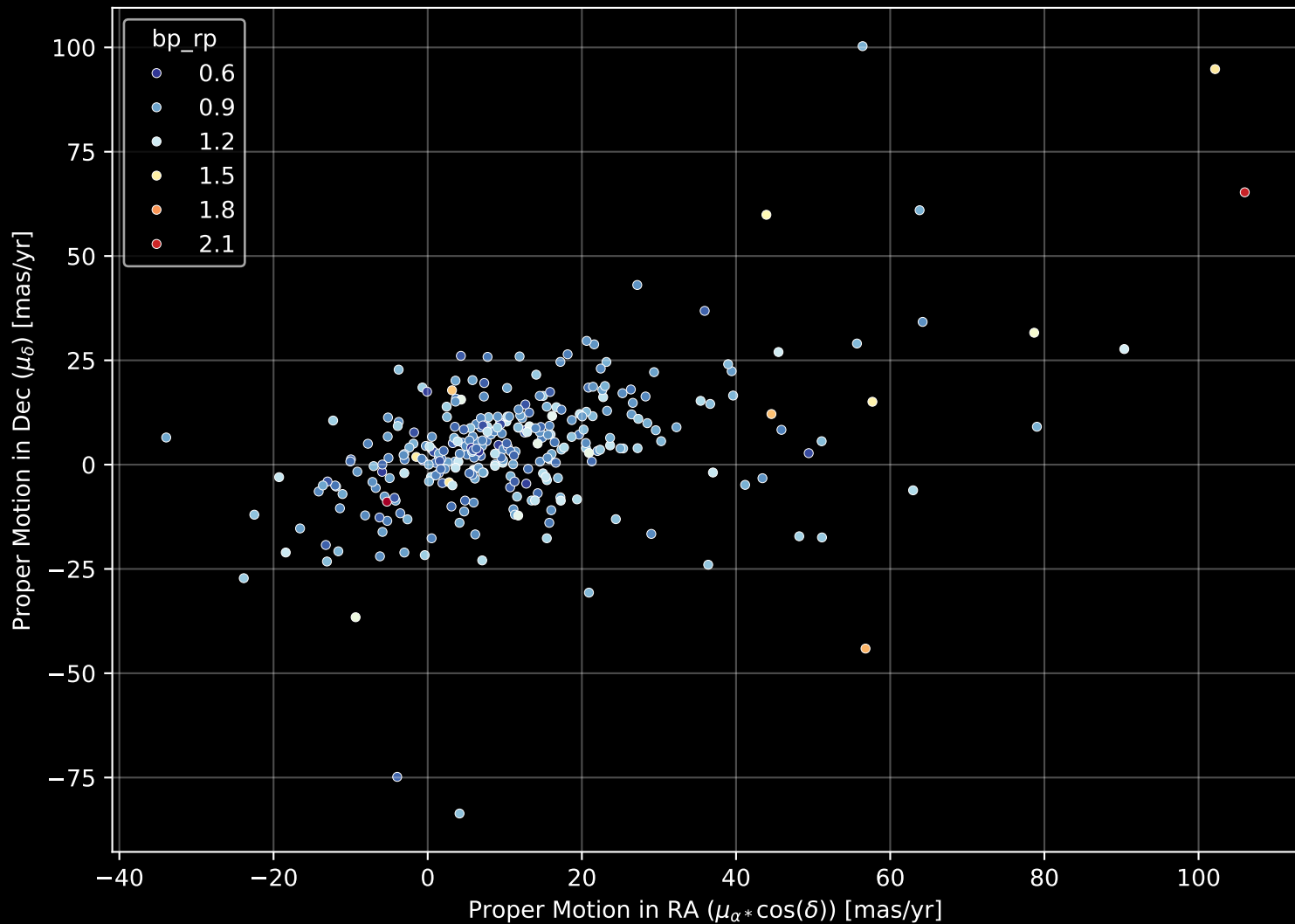
GALAH DR4 Field: [62] Proper Motion Diagram (n= 308)
