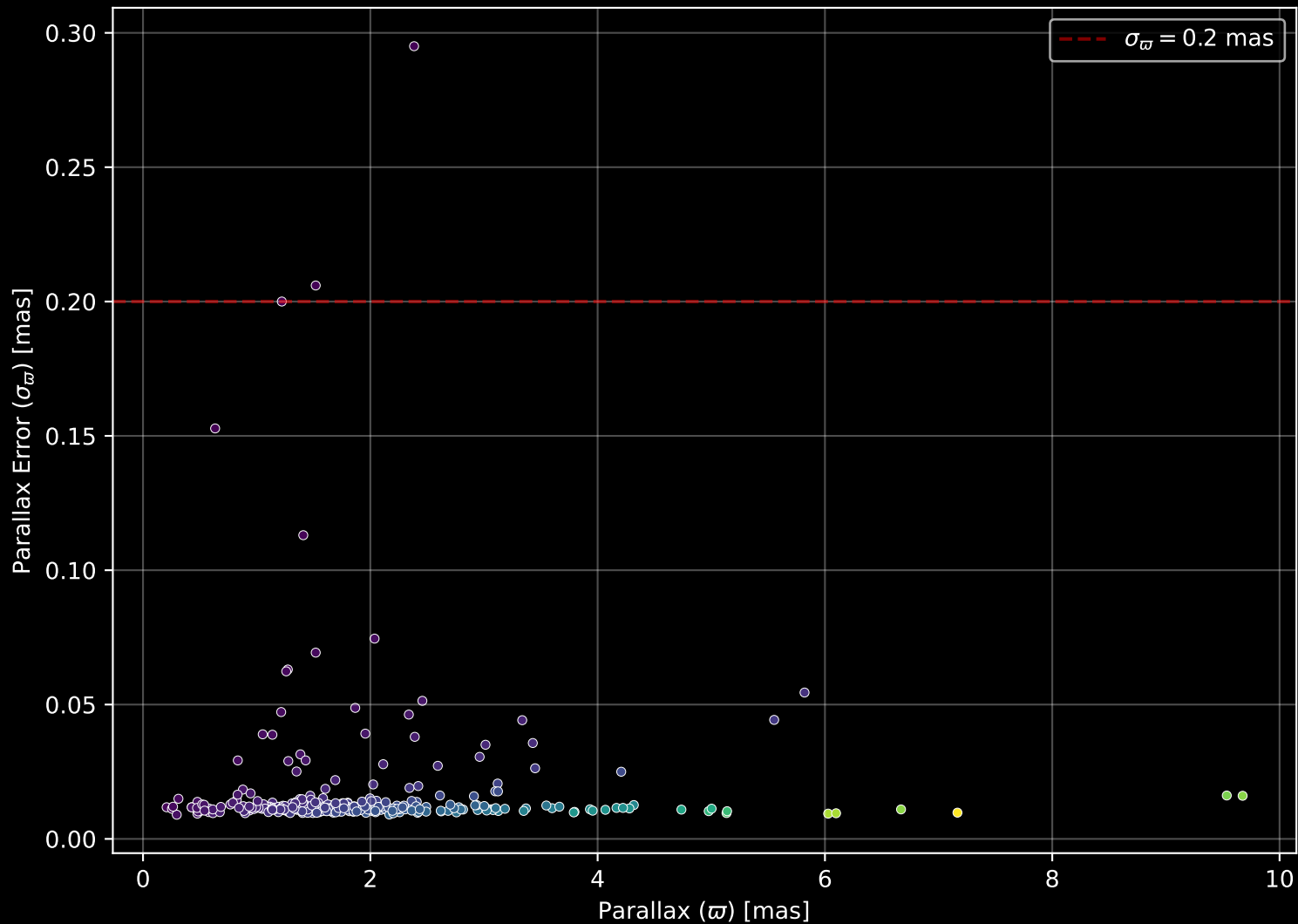
GALAH DR4 Field: [62] Parallax Quality (n= 308)
