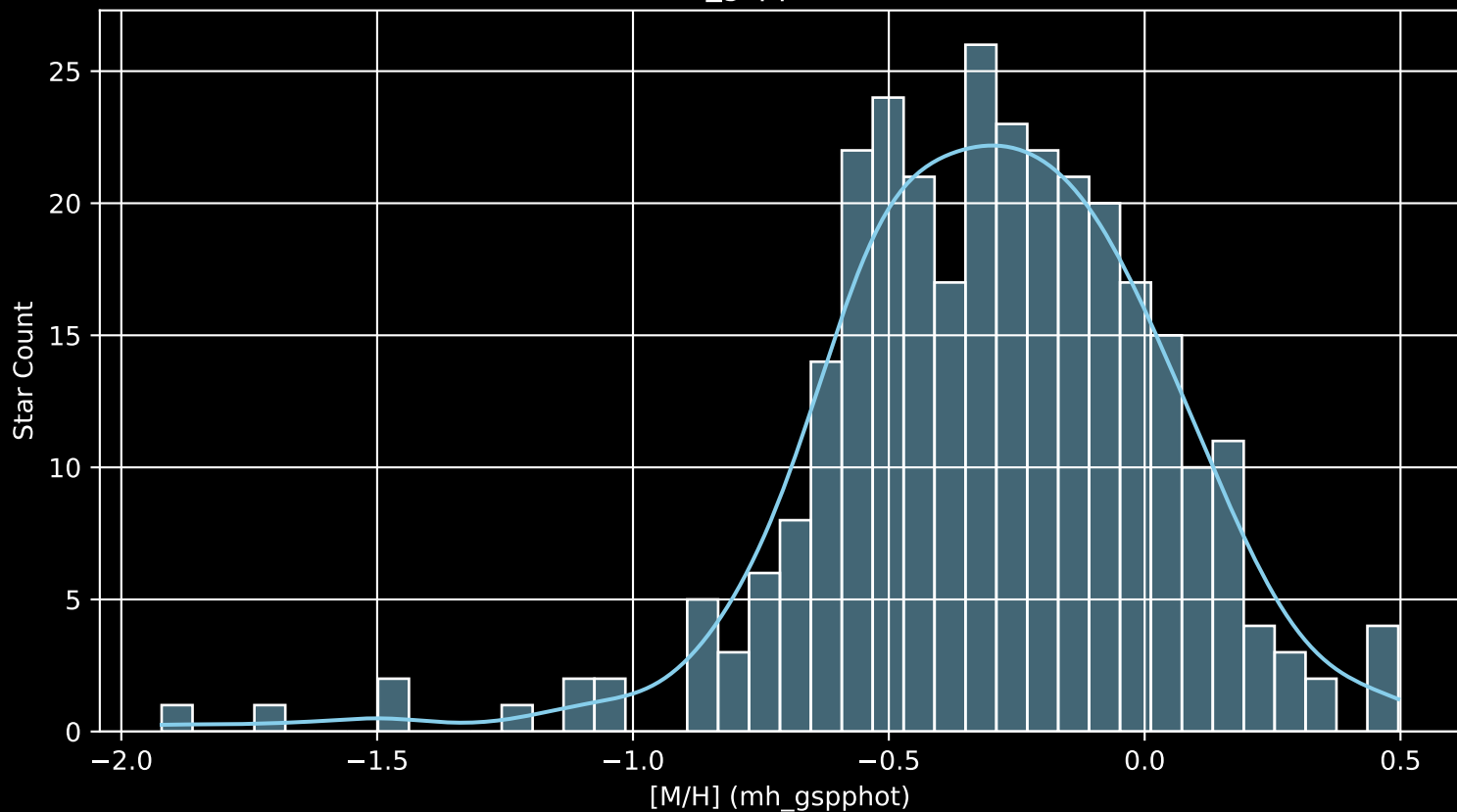
GALAH DR4 Field: [62] [M/H] (mh_gspphot) (n= 307)
