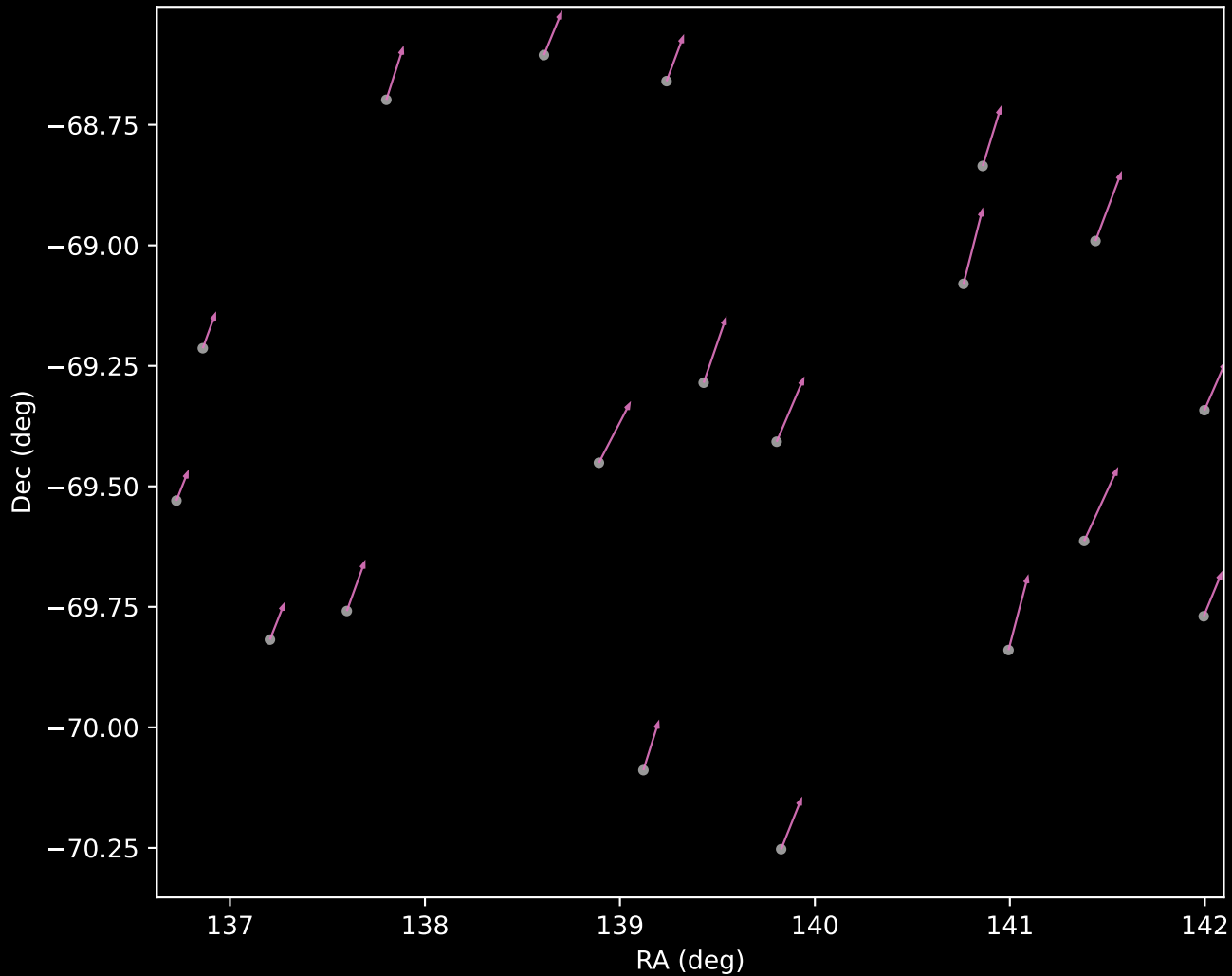
GALAH DR4 Cluster 12 Proper Motion Vectors (n=19)
