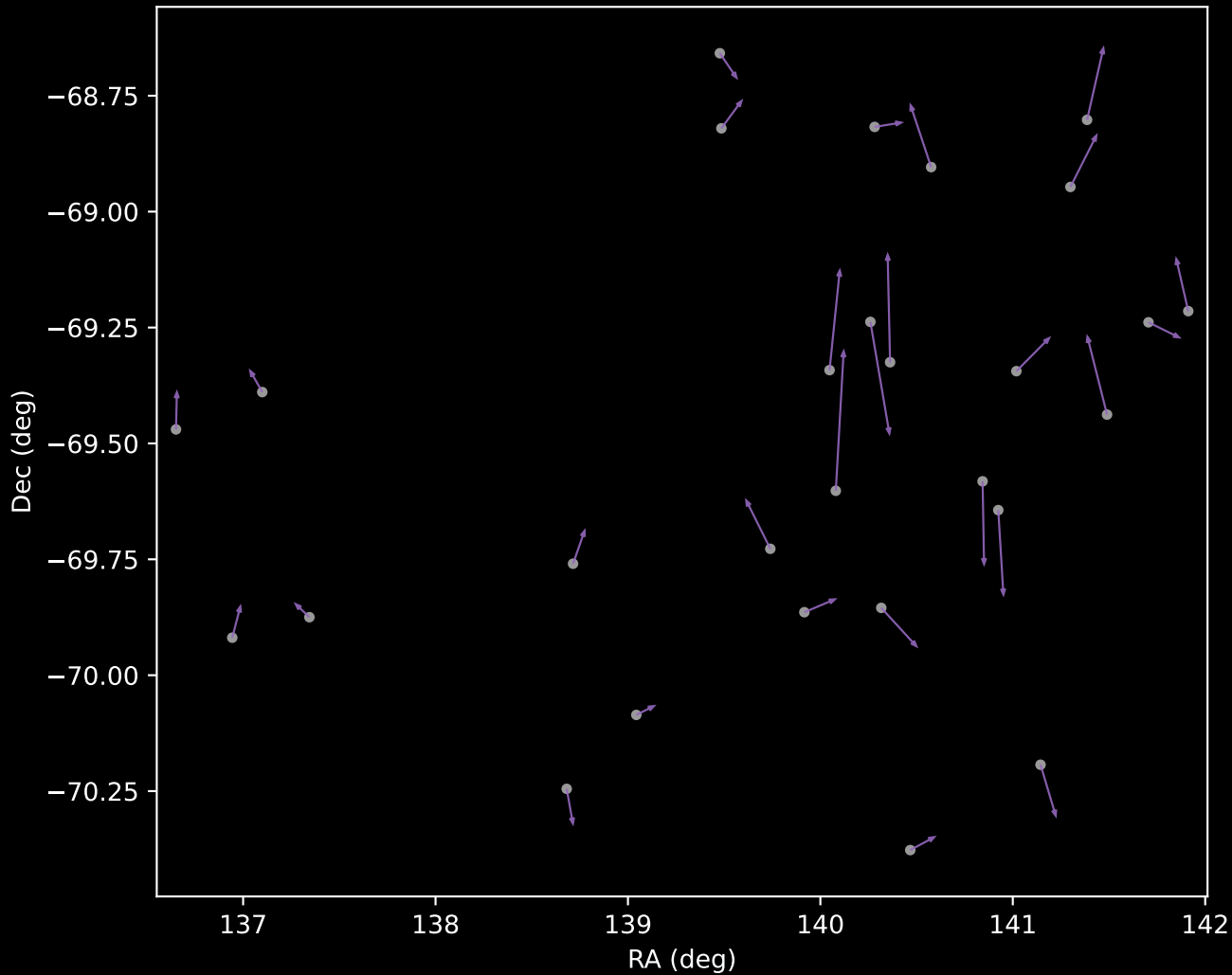
GALAH DR4 Cluster 8 Proper Motion Vectors (n=28)
