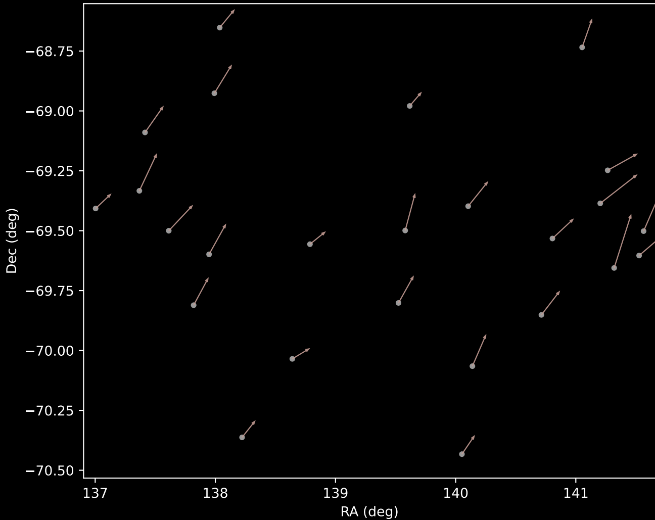
GALAH DR4 Cluster 11 Proper Motion Vectors (n=25)
