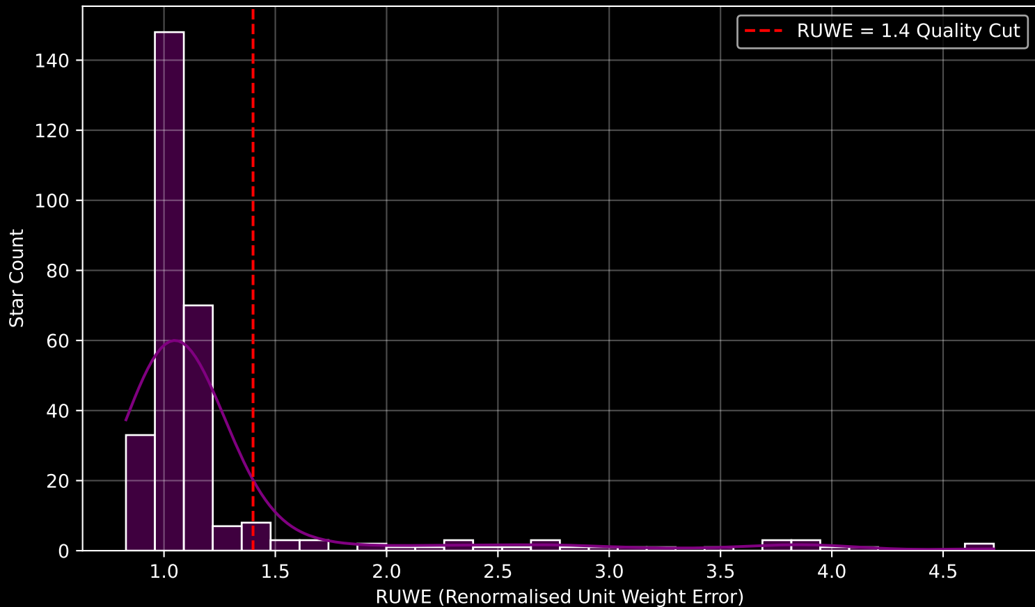
GALAH DR4 Field [62] RUWE Distribution (n= 299)
