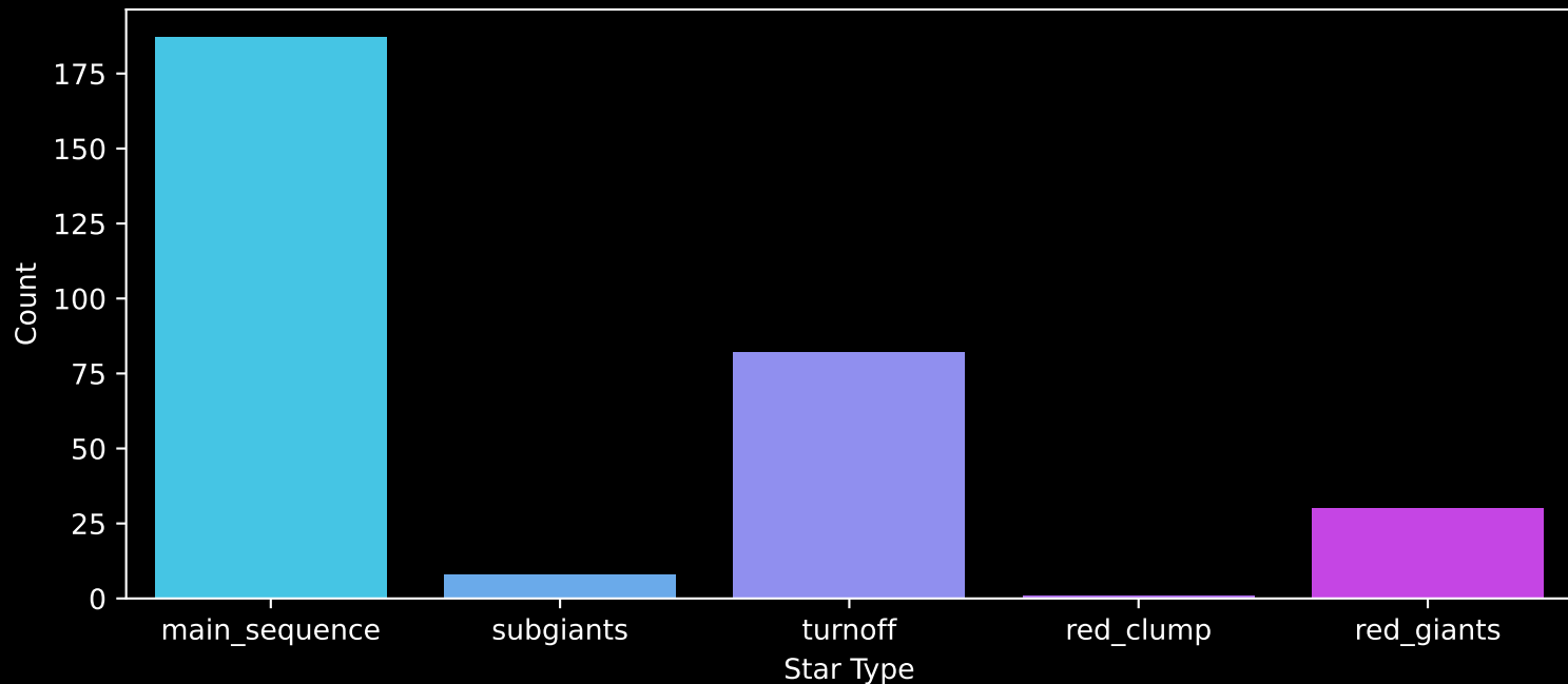
GALAH DR4 Field: [62] Count plot of Star Type
